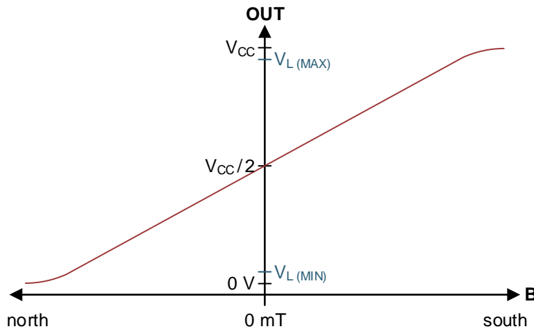
Figure 10. Magnetic Response
