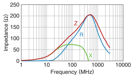
MMZ1608Y121BTD25
