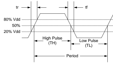
Figure 3. Output Waveform
