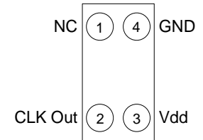
Figure 1. Pin Assignments
