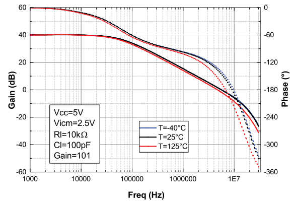
Figure 23. Bode diagram at V_{CC} = 5\text{ V}
