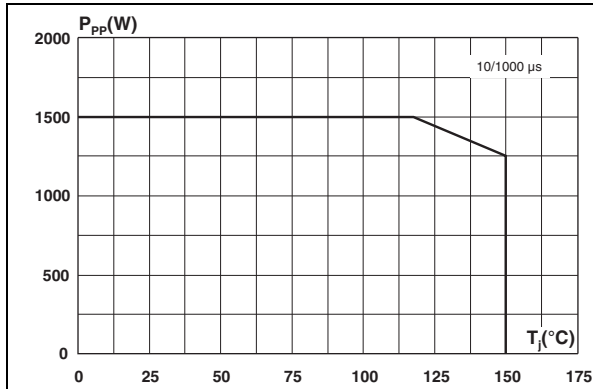
Figure 3. Peak pulse power dissipation versus initial junction temperature (typical values)
