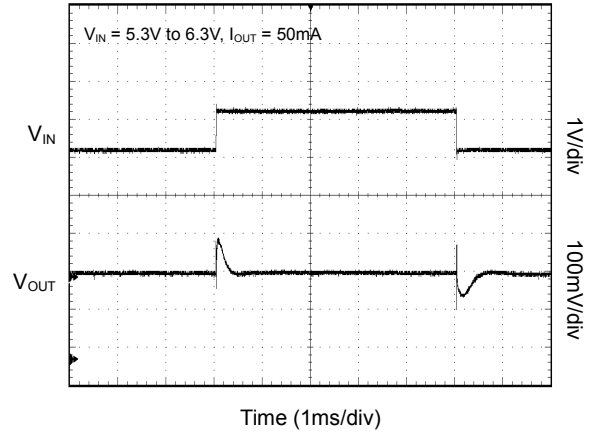
Line-Transient Response
