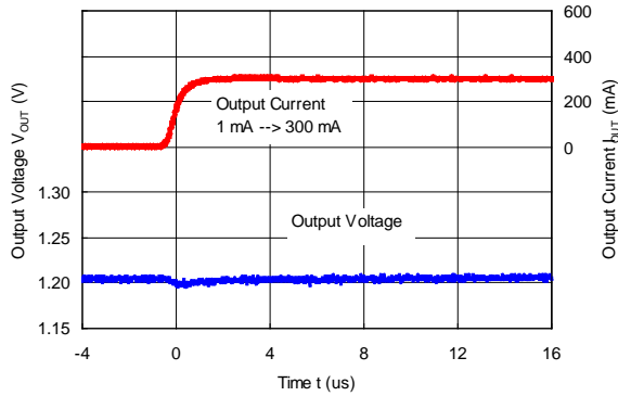
RP508K121x ( V_{IN} = 3.6\text{ V} , V_{OUT} = 1.2\text{ V} ) L = MDT1608CHR47N (1608size_0.47 \mu\text{H} ) MODE = "H" forced PWM control
