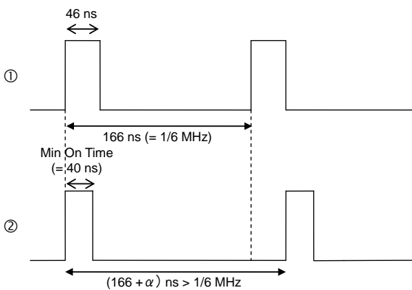
LX Waveform
