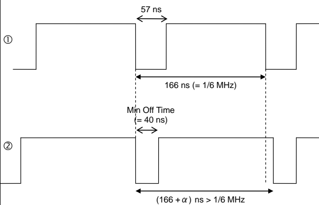
LX Waveform
