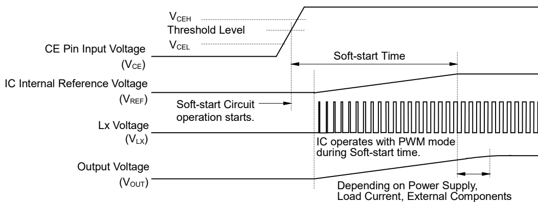
Timing Chart
