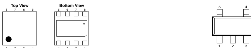
RP402K [DFN(PLP)2020-8] Pin Configurations
