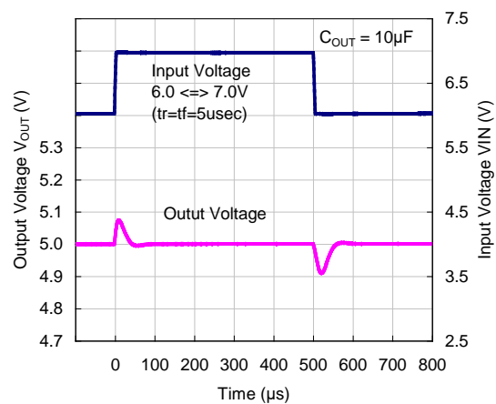
VR=5.0V, I OUT =30mA, C OUT =10μF
