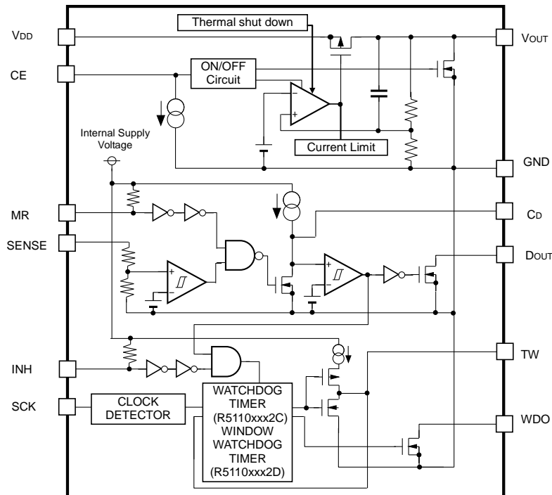
R5110xxx2C / R5110xxx2D
