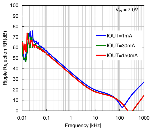
VR=5.0V
