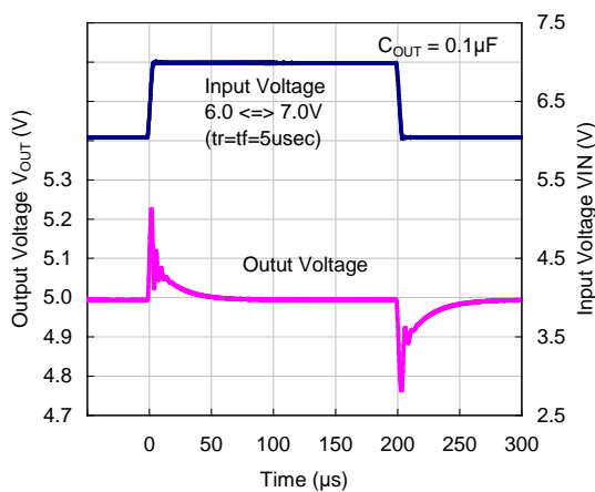
VR=5.0V, I OUT =30mA, C OUT =0.1μF
