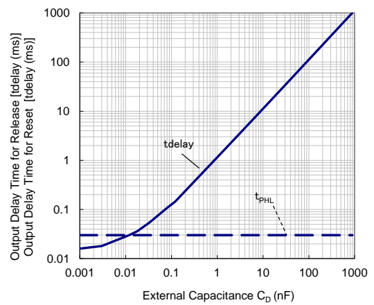
19) Release Output Delay Time External Capacitor and Detect Delay Time vs. for C_D Pin
