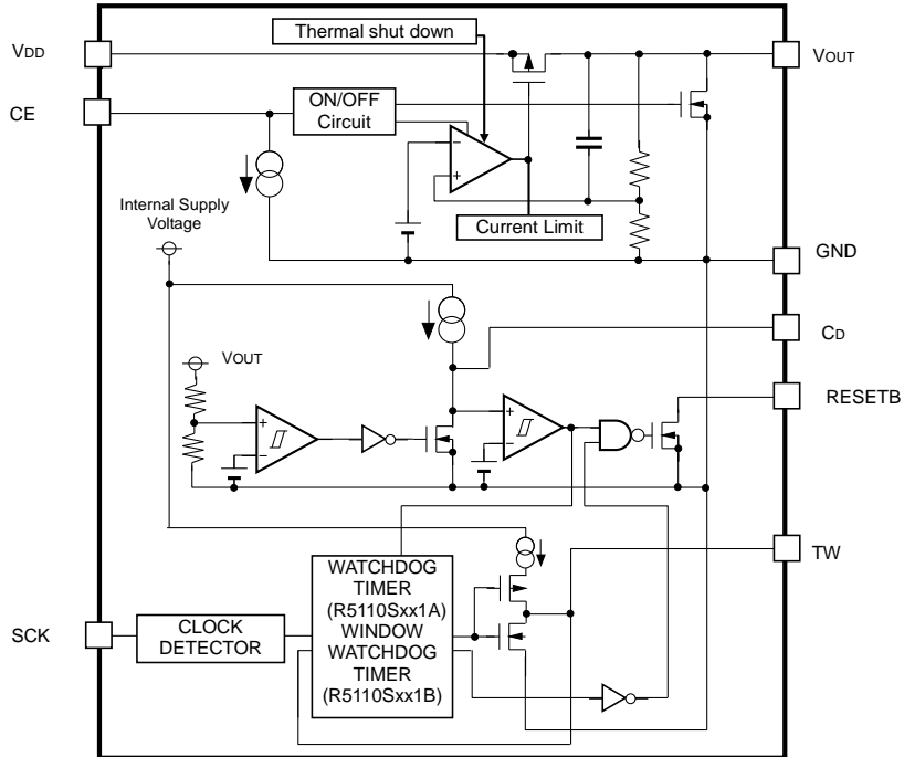
R5110Sxx1A / R5110Sxx1B
