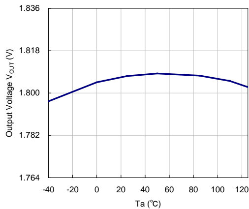
VR=1.8V
