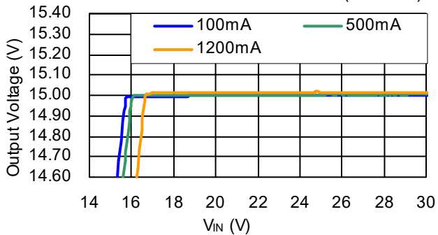
R1245x00xC/R1245x00xD V_{OUT}=15V
