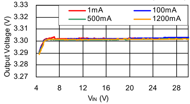
R1245x00xC/R1245x00xD V_{OUT}=3.3V
