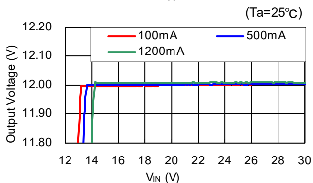
R1245x00xE/R1245x00xF V OUT =12V
