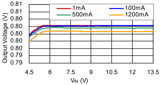
R1245x00xC/R1245x00xD V_{OUT}=0.8V
