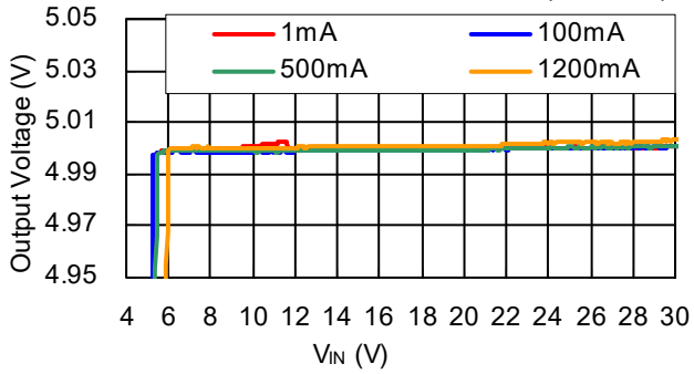
R1245x00xC/R1245x00xD V_{OUT}=5.0V
