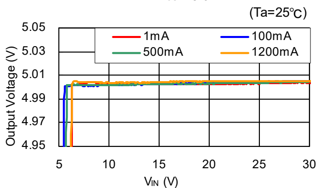
R1245x00xE/R1245x00xF V OUT =5.0V
