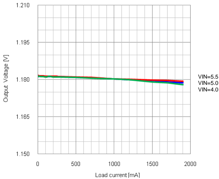
Figure 18. Load regulation PWM mode
