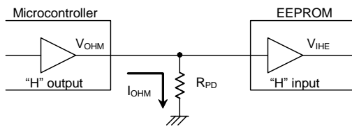
Figure 44. Pull down resistance
