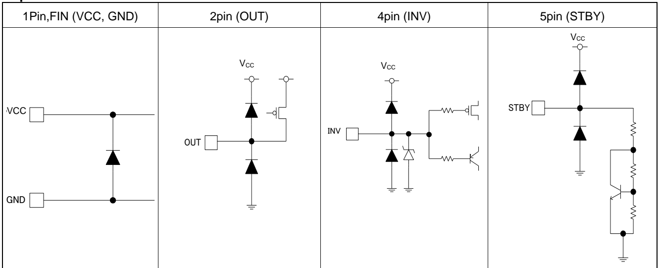
Figure 30. Input Output Equivalent Circuit
