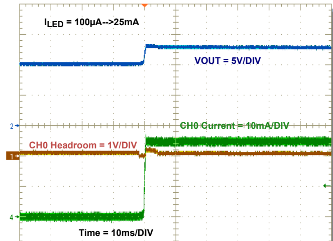
FIGURE 13. TRANSIENT RESPONSE (LED CURRENT CHANGES from 100µA to 25mA)
