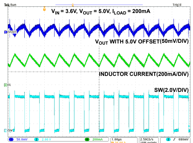
FIGURE 18. PWM WAVEFORM
