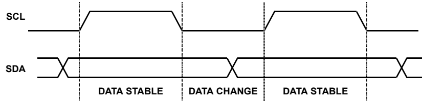
FIGURE 12. VALID DATA CHANGES ON THE SDA BUS
