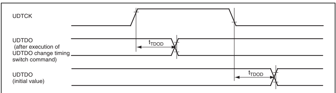
Figure 26.3 H-UDI Data Transfer Timing
