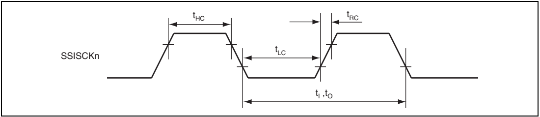
Figure 29.34 Clock Input/Output Timing
