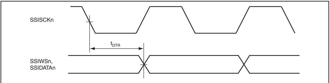
Figure 29.36 SSI Transmit Timing (2)
