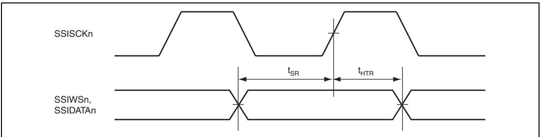
Figure 29.37 SSI Receive Timing (1)
