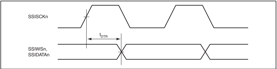
Figure 29.35 SSI Transmit Timing (1)
