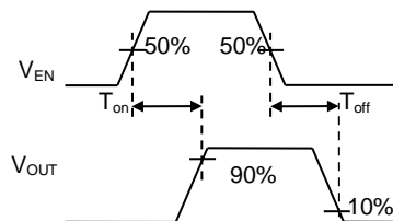
Turn-on Time and Turn-off Time
