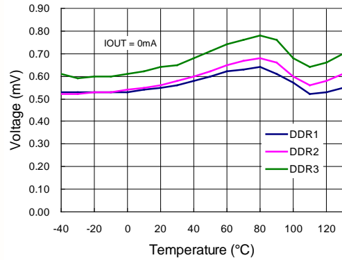
VOS vs. Temperature, VCNTL=5V
