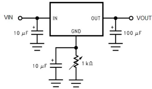
(2) Adjusting Output of Fixed Voltage Regulators
