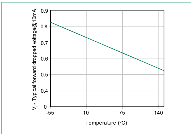
Figure 5 - Forward Voltage
