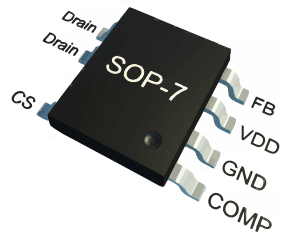
SOP-7
