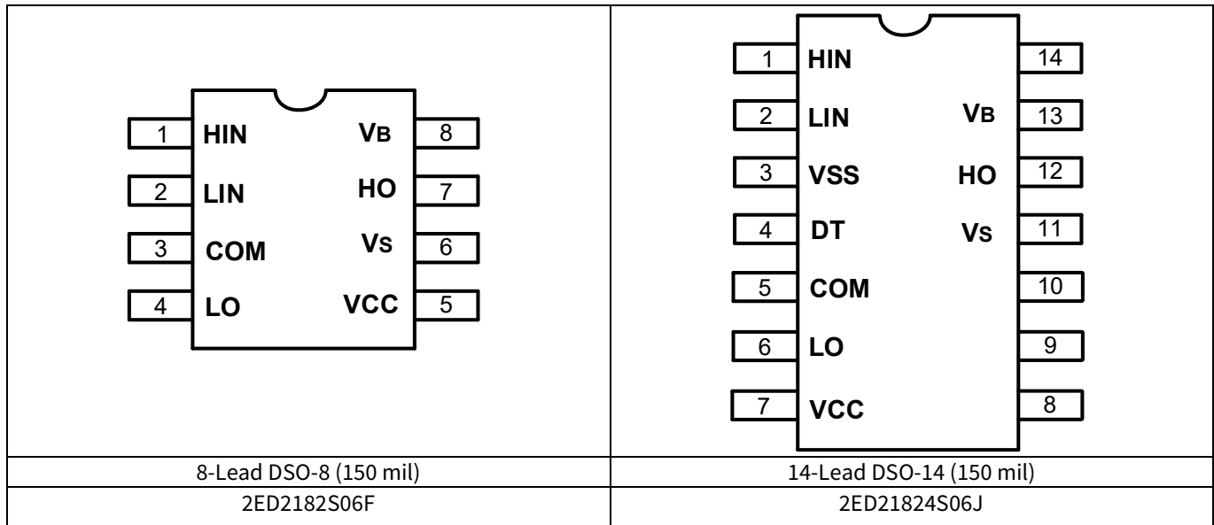
Figure 3 2ED2182(4)S06F(J) pin assignments (top view)
