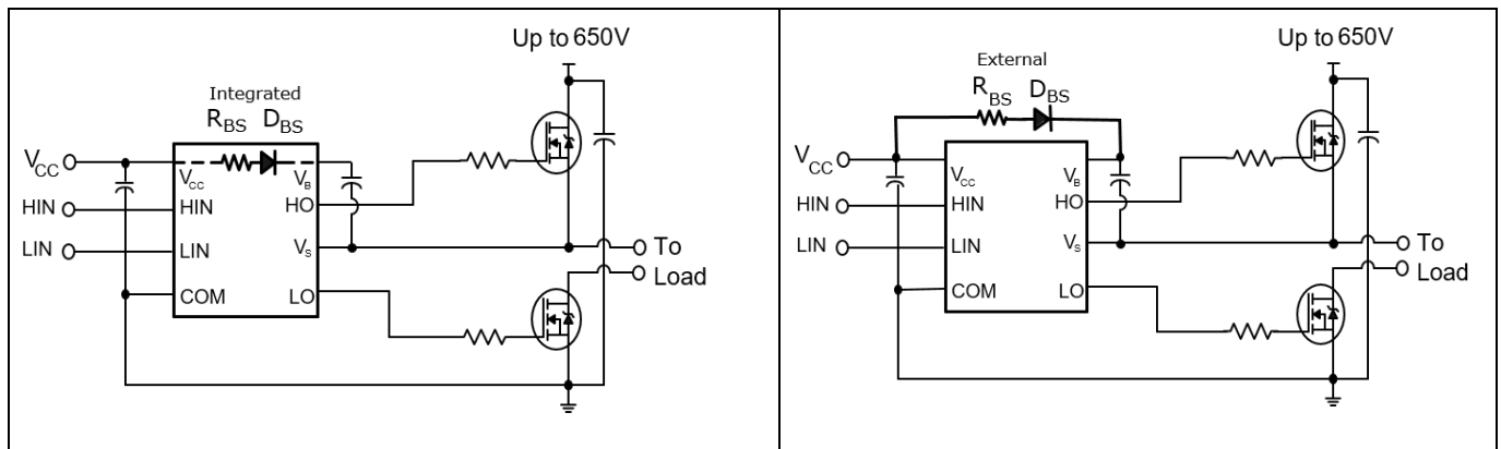
Figure 14 2ED218x with integrated components
