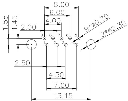
RECOMMENDER P.C.B.LAYOUT TOP VIEW (COMPONENT SIDE TOLERANCE±0.05)
