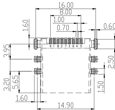
RECOMMEND PCB LAYOUT(±0.05)
