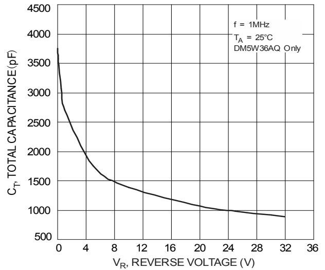
Fig. 6 Typical Total Capacitance
