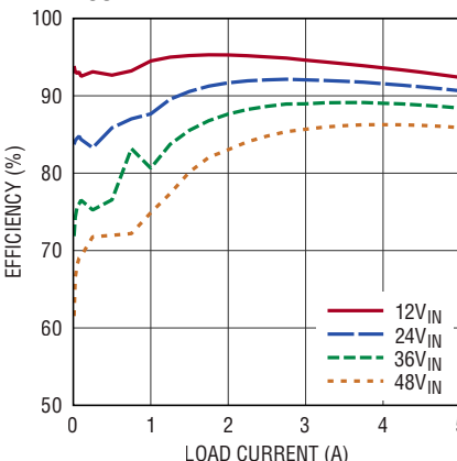
Efficiency vs Load Current V_{OUT} = 5\text{V} , BIAS = 5V
