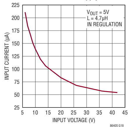
LT8643S No-Load Supply Current
