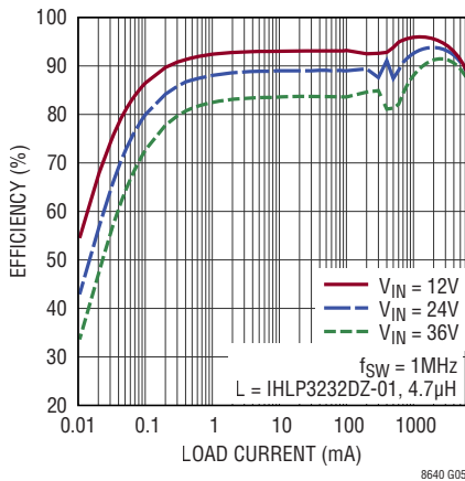
LT8640S Low Load Efficiency at 5V OUT
