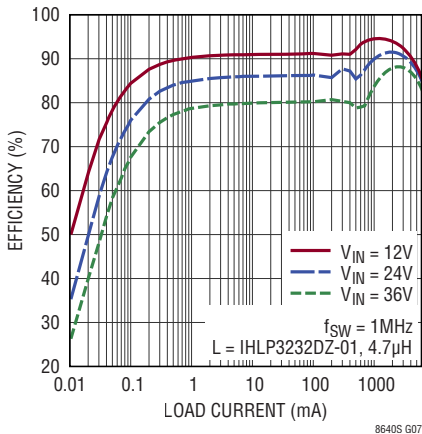
LT8640S Low Load Efficiency at 3.3V OUT
