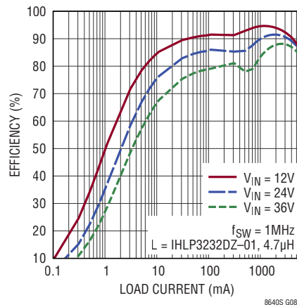
LT8643S Low Load Efficiency at 3.3V OUT
