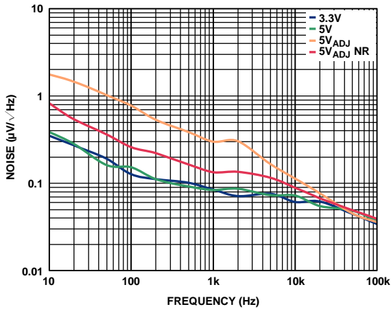
图49. 输出噪声频谱密度( I_{LOAD} = 10 mA , C_{OUT} = 1 \mu F )
