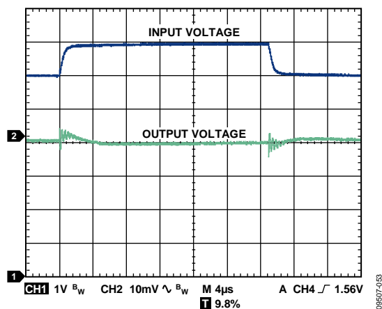
图58.线路瞬态响应( C_{IN} 、 C_{OUT} = 1 \mu\text{F} , I_{LOAD} = 1 \text{ mA} , V_{OUT} = 5 \text{ V} )
