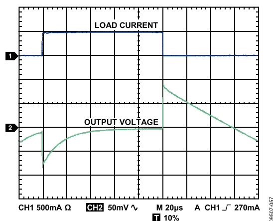
图62. 输出瞬态响应( V_{\text{OUT}} = 1.8\ \text{V} , C_{\text{OUT}} = 1\ \mu\text{F} )
