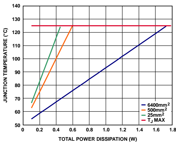
图71. LFCSP, T_A = 50^\circ\text{C}
