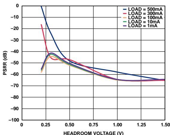
图46. 电源抑制比与裕量电压的关系(10 kHz, V_{OUT} = 5V )
