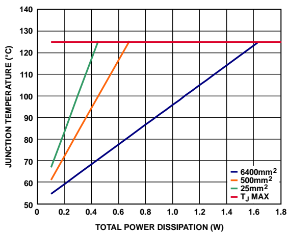
图74. SOIC, T_A = 50^\circ\text{C}
