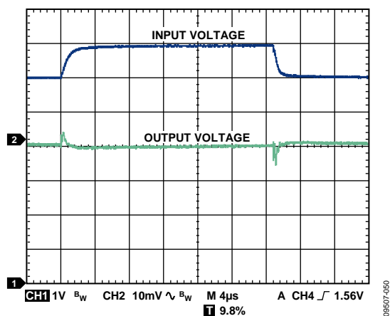
图55.线路瞬态响应( C_{IN} 、 C_{OUT} = 1 \mu\text{F} , I_{LOAD} = 500 \text{ mA} , V_{OUT} = 5 \text{ V} )
