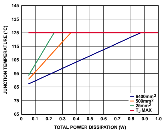
图75. SOIC, T_A = 85^\circ\text{C}
