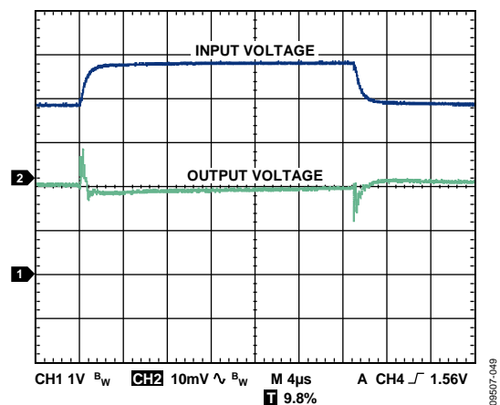
图54.线路瞬态响应( C_{IN} 、 C_{OUT} = 1 \mu\text{F} , I_{LOAD} = 500 \text{ mA} , V_{OUT} = 3.3 \text{ V} )
