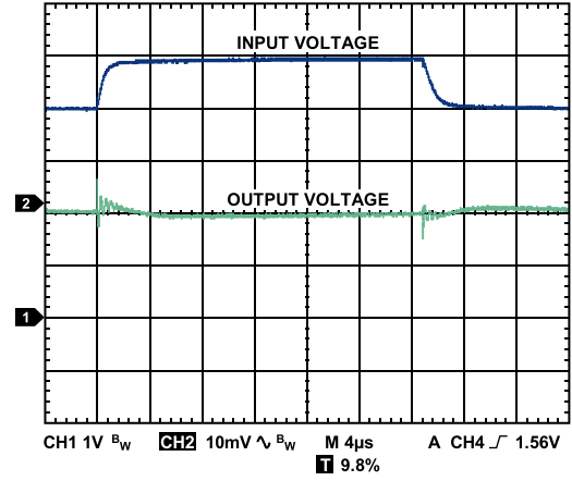
图50. 负载瞬态响应( C_{IN} 、 C_{OUT} = 1 \mu F , I_{LOAD} = 1 mA 至 500 mA, V_{OUT} = 1.8 V , V_{IN} = 5 V )
