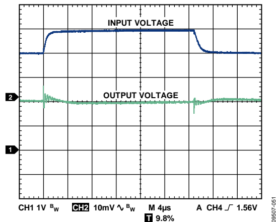
图56.线路瞬态响应( C_{IN} 、 C_{OUT} = 1 \mu\text{F} , I_{LOAD} = 1 \text{ mA} , V_{OUT} = 1.8 \text{ V} )
