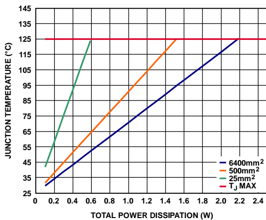
图73. SOIC, T_A = 25^\circ\text{C}
