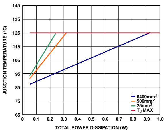
图72. LFCSP, T_A = 85^\circ\text{C}
