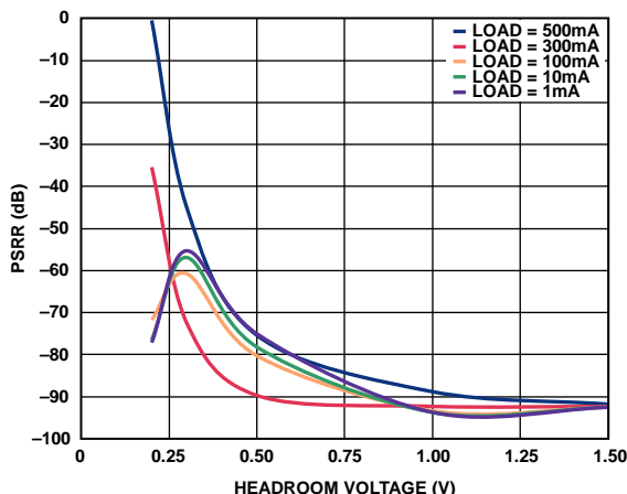
图45. 电源抑制比与裕量电压的关系(1 kHz, V_{OUT} = 5V )
