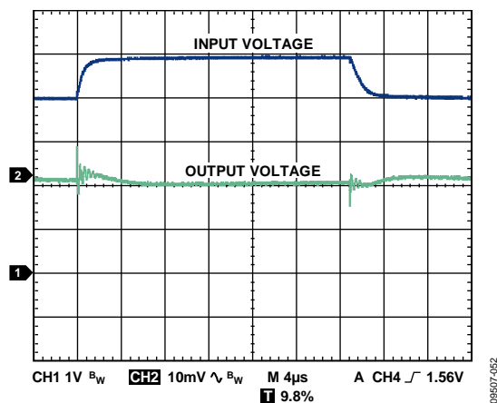
图57.线路瞬态响应( C_{IN} 、 C_{OUT} = 1 \mu\text{F} , I_{LOAD} = 1 \text{ mA} , V_{OUT} = 3.3 \text{ V} )
