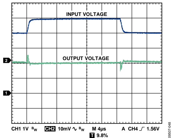
图53.线路瞬态响应( C_{IN} 、 C_{OUT} = 1 \mu\text{F} , I_{LOAD} = 500 \text{ mA} , V_{OUT} = 1.8 \text{ V} )
