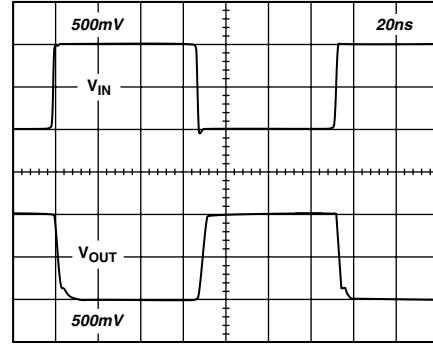
TPC 27. Small Signal Pulse Response, Gain = -1 ( R_{FB} = 909 \Omega , R_L = 150 \Omega , V_S = \pm 7.5 \text{ V} )
