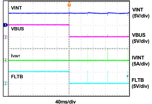
Figure 13. Short-Circuit Protection ( V_{INT} = 5\text{V} , R_{LIM} = 30\text{k}\Omega ) (Auto-Restart)
