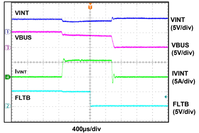
Figure 11. Over-Current Protection ( V_{INT} = 5\text{V} , R_{LIM} = 30\text{k}\Omega )
