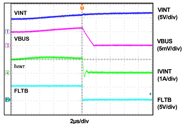
Figure 9. VINT OVP operation with R_{OVP} = 180\text{k}\Omega
