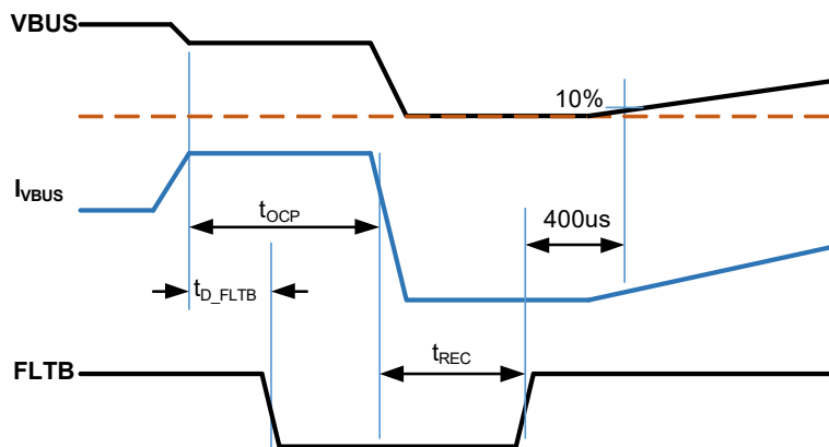
Figure 3. OCP and FLT Time
