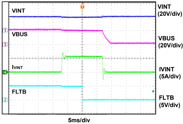
Figure 10. Over-Current Protection ( V_{INT} = 20\text{V} , R_{LIM} = 30\text{k}\Omega )
