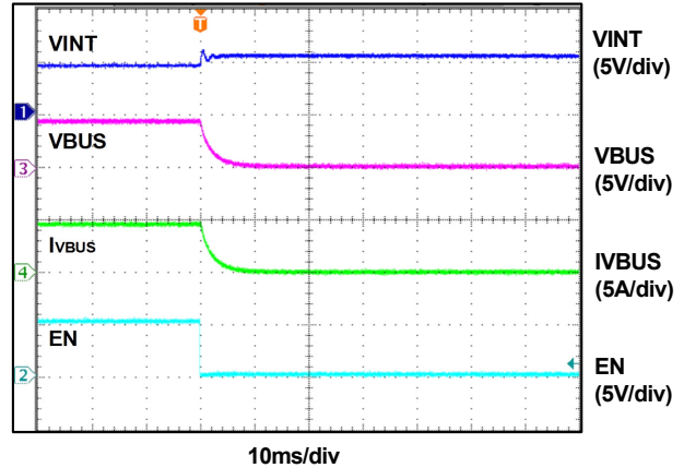
Figure 7. Turn-Off by EN (VINT = 5V)
