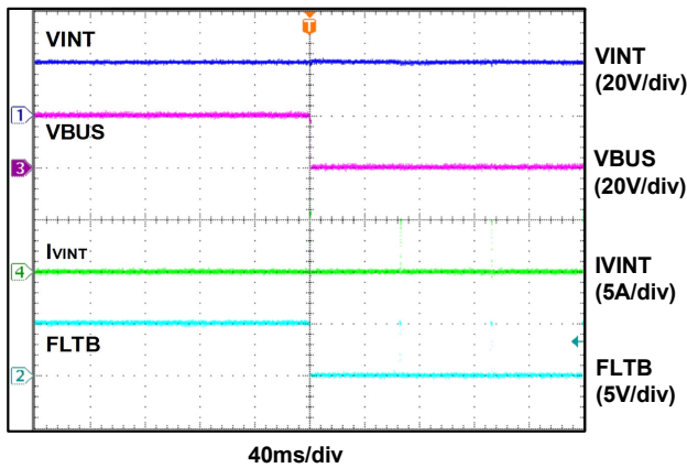
Figure 12. Short-Circuit Protection ( V_{INT} = 20\text{V} , R_{LIM} = 30\text{k}\Omega ) (Auto-Restart)
