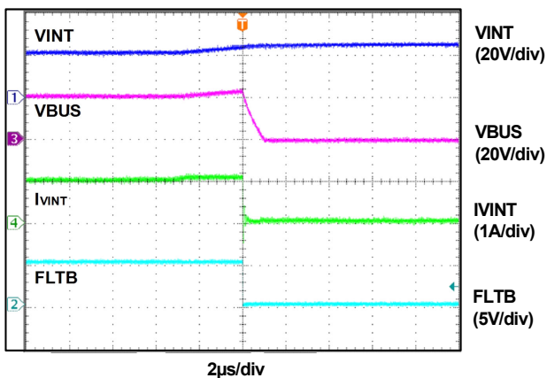
Figure 8. VINT OVP operation with R_{OVP} = 20\text{k}\Omega
