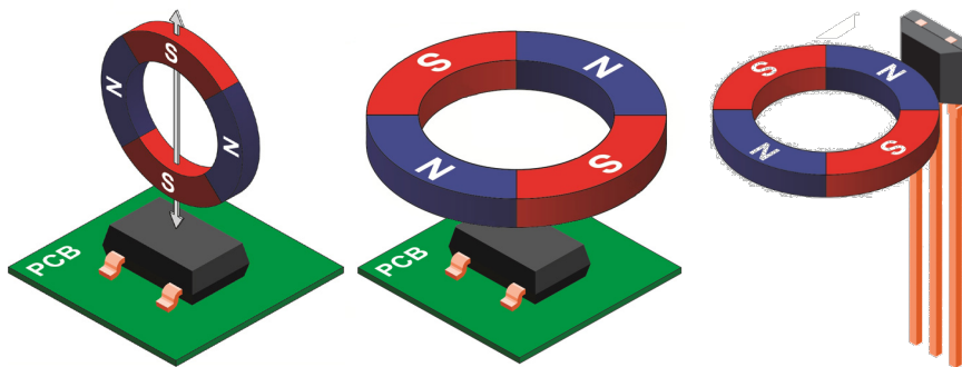
Figure 5: Sensing Configurations
