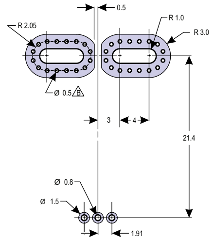
\triangle PCB Layout Reference View
