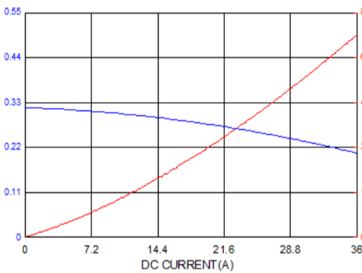
ASPIAIG-F7020-R68
