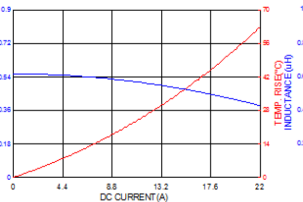
ASPIAIG-F5020-R47
