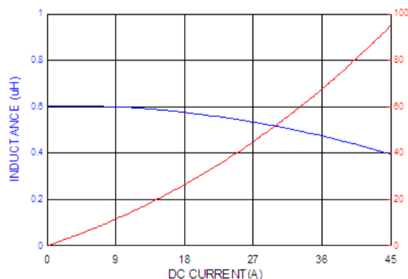
ASPIAIG-F7030-R60
