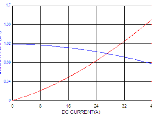
ASPIAIG-F7030-1R0
