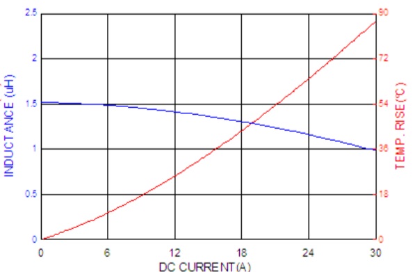
ASPIAIG-F7030-1R5
