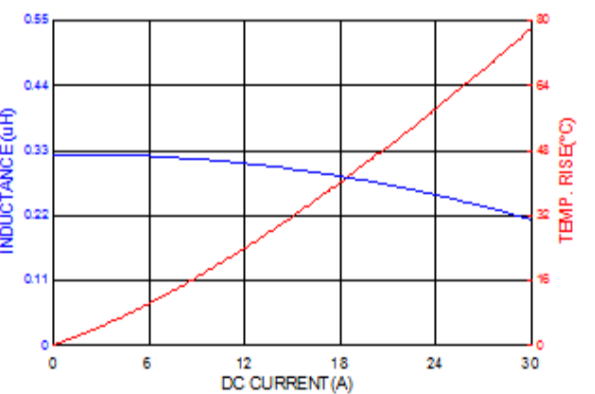
ASPIAIG-F5020-R68
