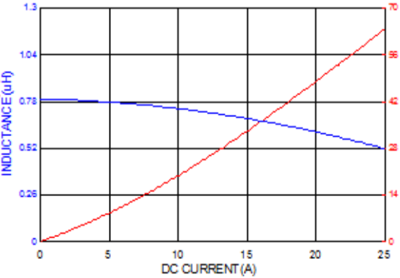
ASPIAIG-F5030-R80
