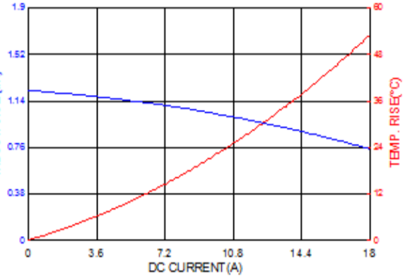
ASPIAIG-F5030-1R2
