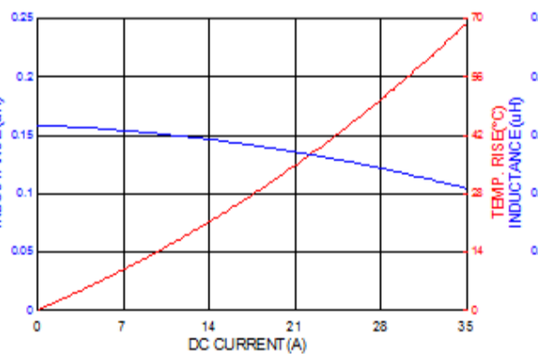
ASPIAIG-F5020-R47
