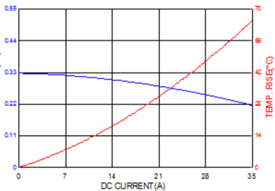
ASPIAIG-F5030-R33
