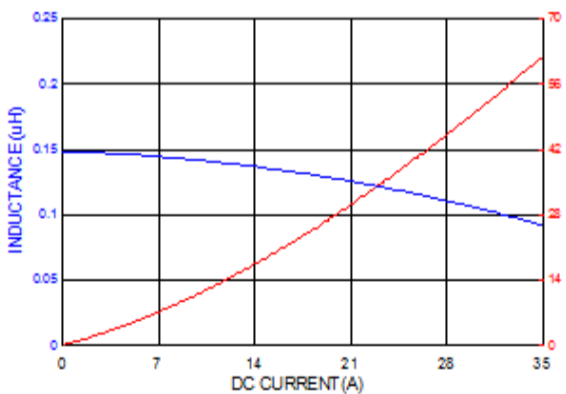
ASPIAIG-F5030-R15
