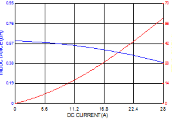
ASPIAIG-F5030-R60
