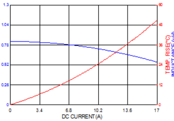
ASPIAIG-F5020-1R5
