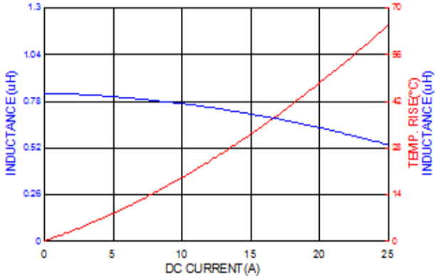
ASPIAIG-F5030-R82
