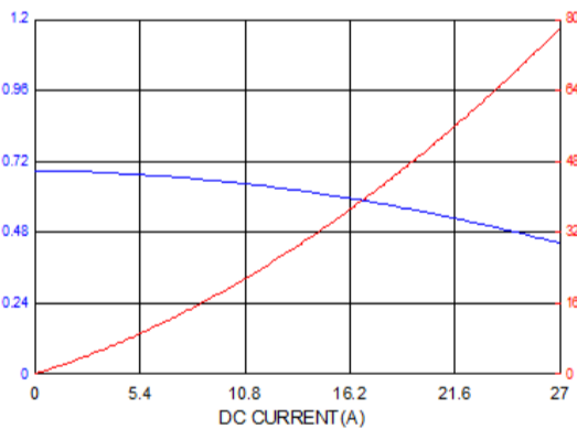
ASPIAIG-F7020-R68
