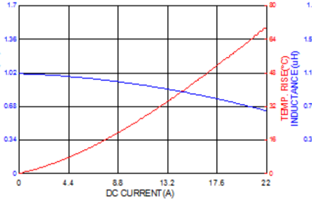
ASPIAIG-F5030-1R0
