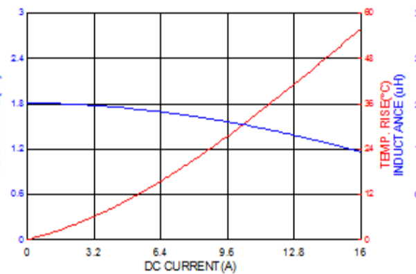
ASPIAIG-F5030-1R8
