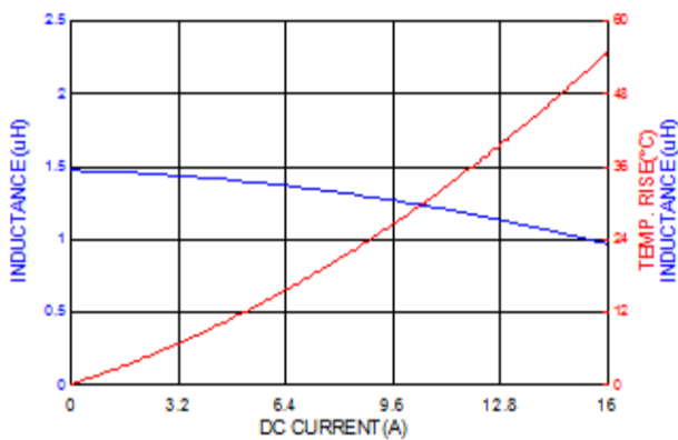
ASPIAIG-F5030-1R5
