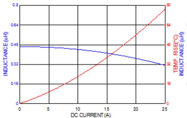
ASPIAIG-F5020-R47
