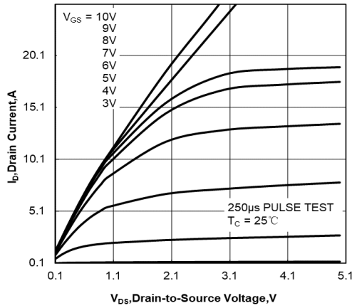
Figure 1. Output Characteristics
