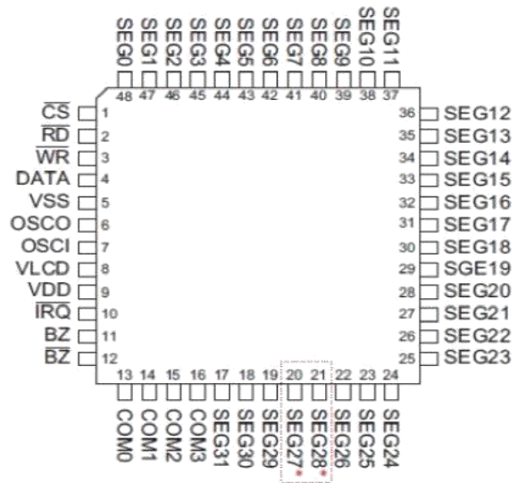
HT1621B 48LQFN
