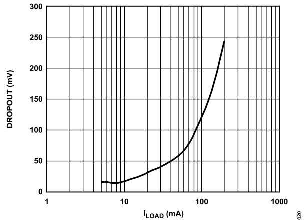
Figure 22. Dropout Voltage ( V_{DROPOUT} ) vs. Load Current ( I_{LOAD} ), V_{OUT} = 3.3\text{ V}
