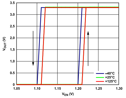
Figure 46. Typical VOUT Response to EN Pin Operation
