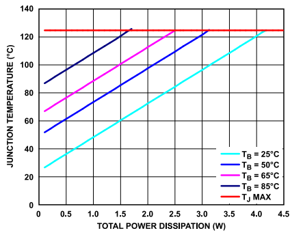
Figure 55. SOIC, T_A = 25^\circ\text{C}
