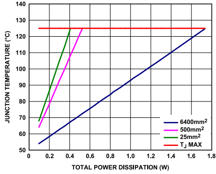
Figure 53. LFCSP, T_A = 50^\circ\text{C}
