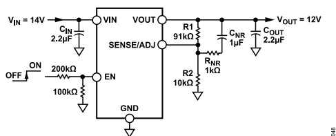
Figure 50. Noise Reduction Modification
