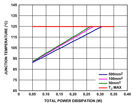
Figure 60. TSOT, T_A = 85^\circ\text{C}
