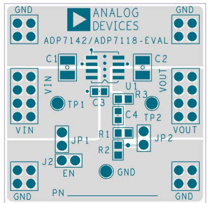
Figure 65. Example SOIC PCB Layout
