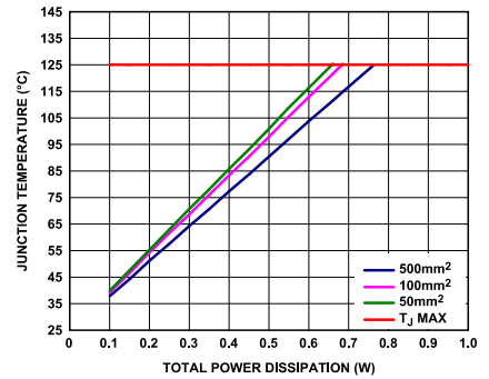
Figure 58. TSOT, T_A = 25^\circ\text{C}
