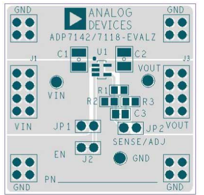
Figure 66. Example TSOT PCB Layout
