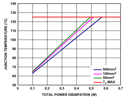
Figure 59. TSOT, T_A = 50^\circ\text{C}
