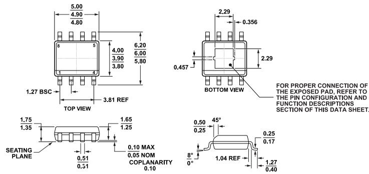
Figure 68. 8-Lead Standard Small Outline Package, with Exposed Pad [SOIC_N_EP] Narrow Body (RD-8-1) Dimensions shown in millimeters
