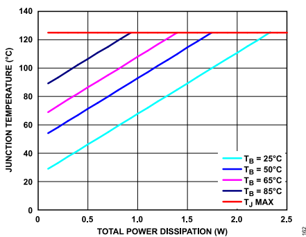
Figure 63. TSOT Junction Temperature Rise, Different Board Temperatures
