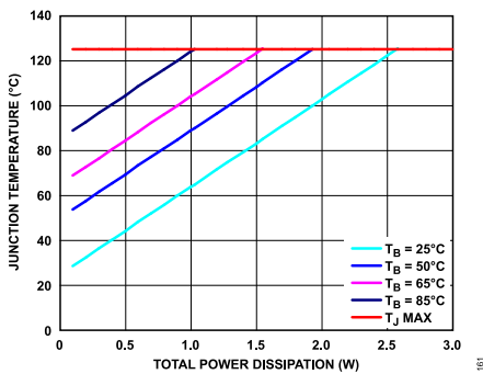
Figure 62. SOIC Junction Temperature Rise, Different Board Temperatures
