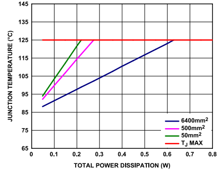
Figure 57. SOIC, T_A = 85^\circ\text{C}
