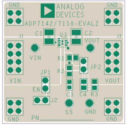
Figure 64. Example LFCSP PCB Layout
