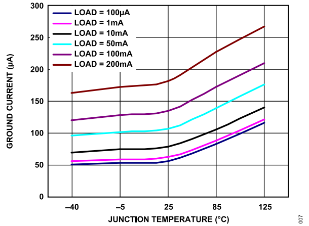
Figure 9. Ground Current ( I_{GND} ) vs. Junction Temperature ( T_J )
