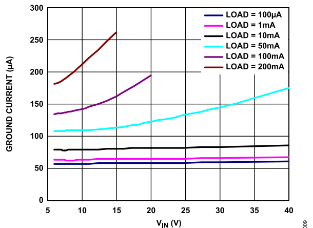
Figure 11. Ground Current ( I_{GND} ) vs. Input Voltage ( V_{IN} )
