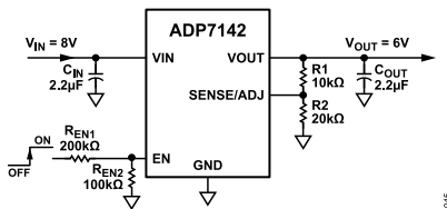
Figure 47. Typical EN Pin Voltage Divider
