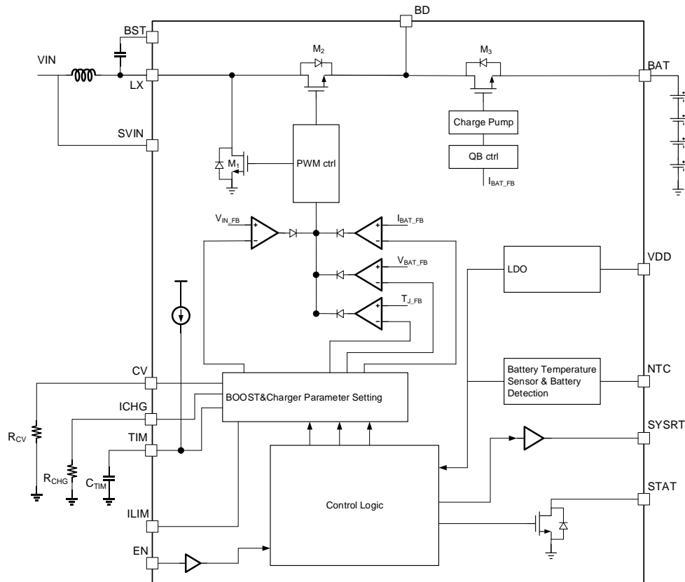
Figure 4. Internal function block diagram
