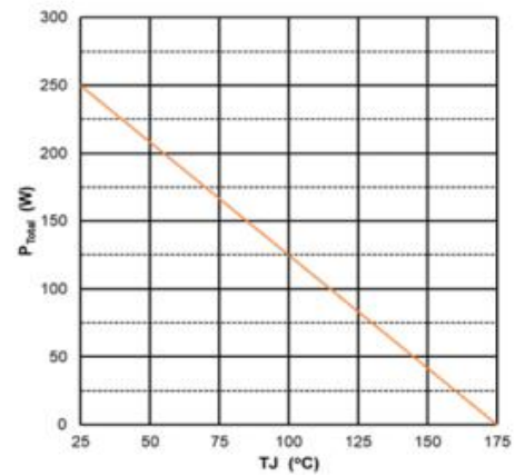
Figure 4. Power Derating
