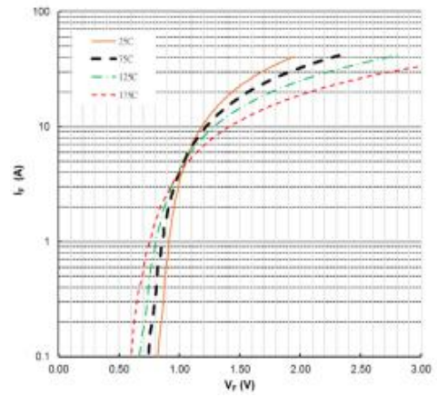
Figure 2. Forward Characteristics
