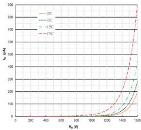
Figure 3. Reverse Characteristics
