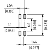
◆ P. C. B LAYOUT
