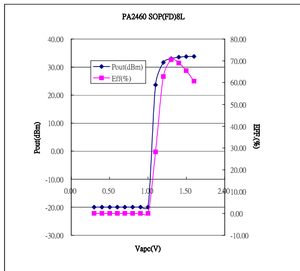
Fig 2.4 Power Output vs. Control Voltage
