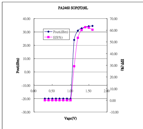
Fig 1.4 Power Output vs. Control Voltage
