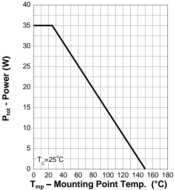
Power Capability
