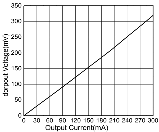
Droop Voltage vs. Output Current
