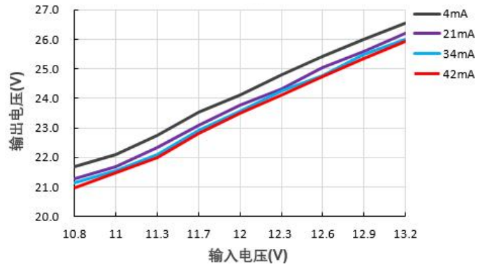
输出电压 VS 输入电压 (B1224S-1W)
