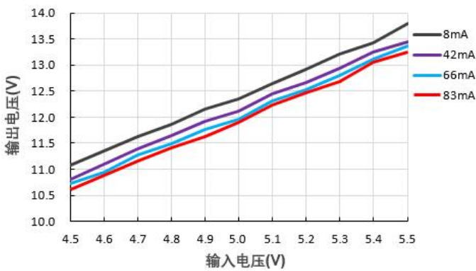
输出电压 VS 输入电压 (B0512S-1W)
