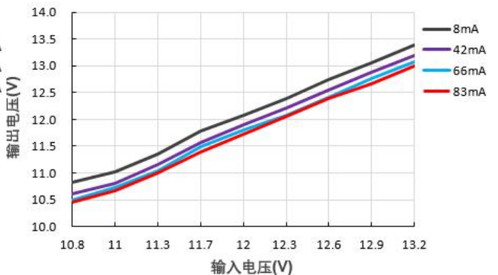
输出电压 VS 输入电压 (B1212S-1W)
