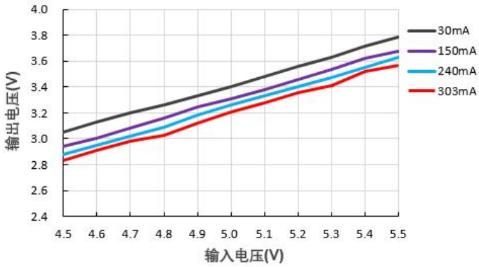
输出电压 VS 输入电压 (B0503S-1W)
