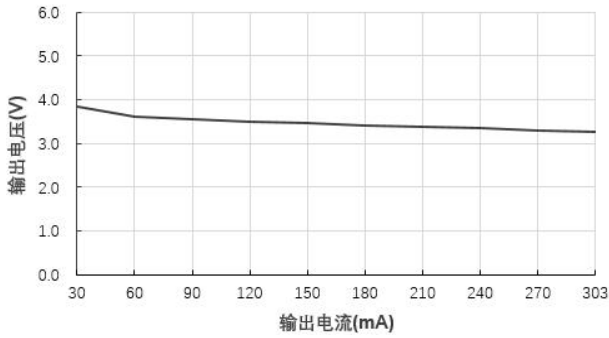
输出电压 VS 输出电流 (B0303S-1W@Vin=3.3V)
