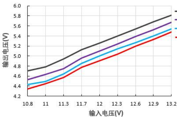
输出电压 VS 输入电压 (B1205S-1W)
