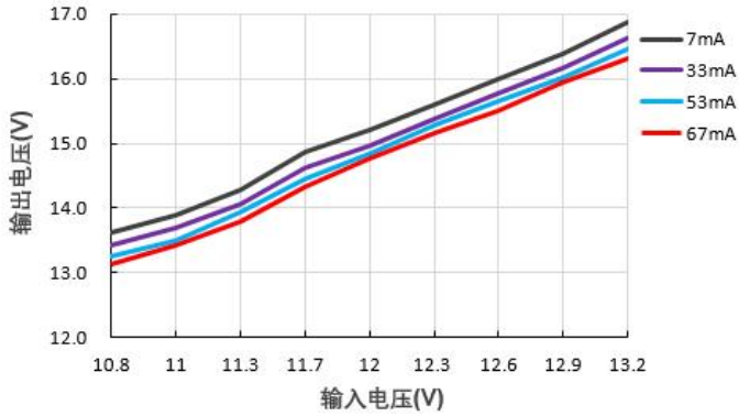
输出电压 VS 输入电压 (B1215S-1W)
