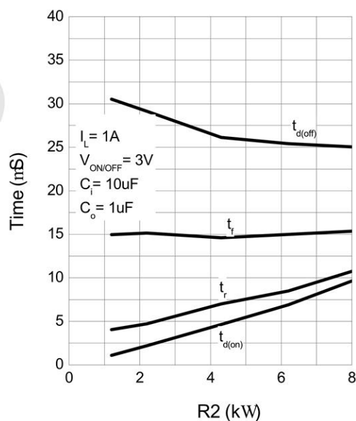
Switching Variation
