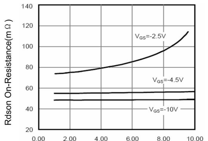
Figure 6 Drain-Source On-Resistance
