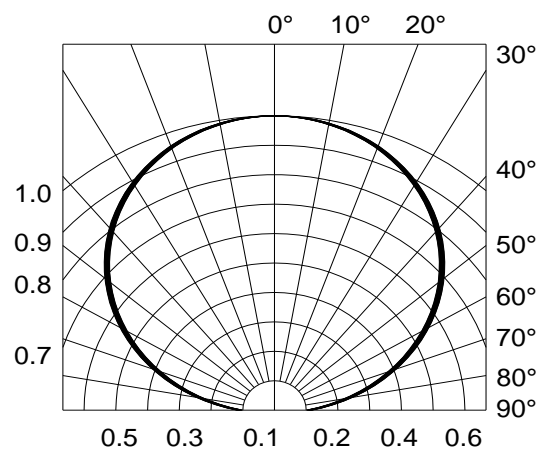
Fig.6-Radiation Diagram Ta=25°C
