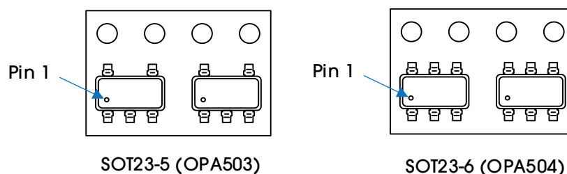
Figure 38. Product Loading Orientation
